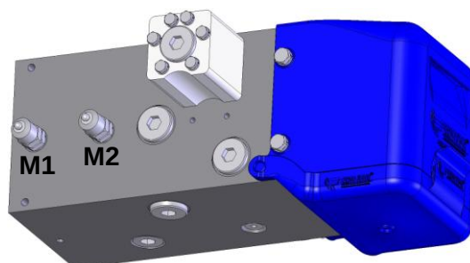
Control valve 02
